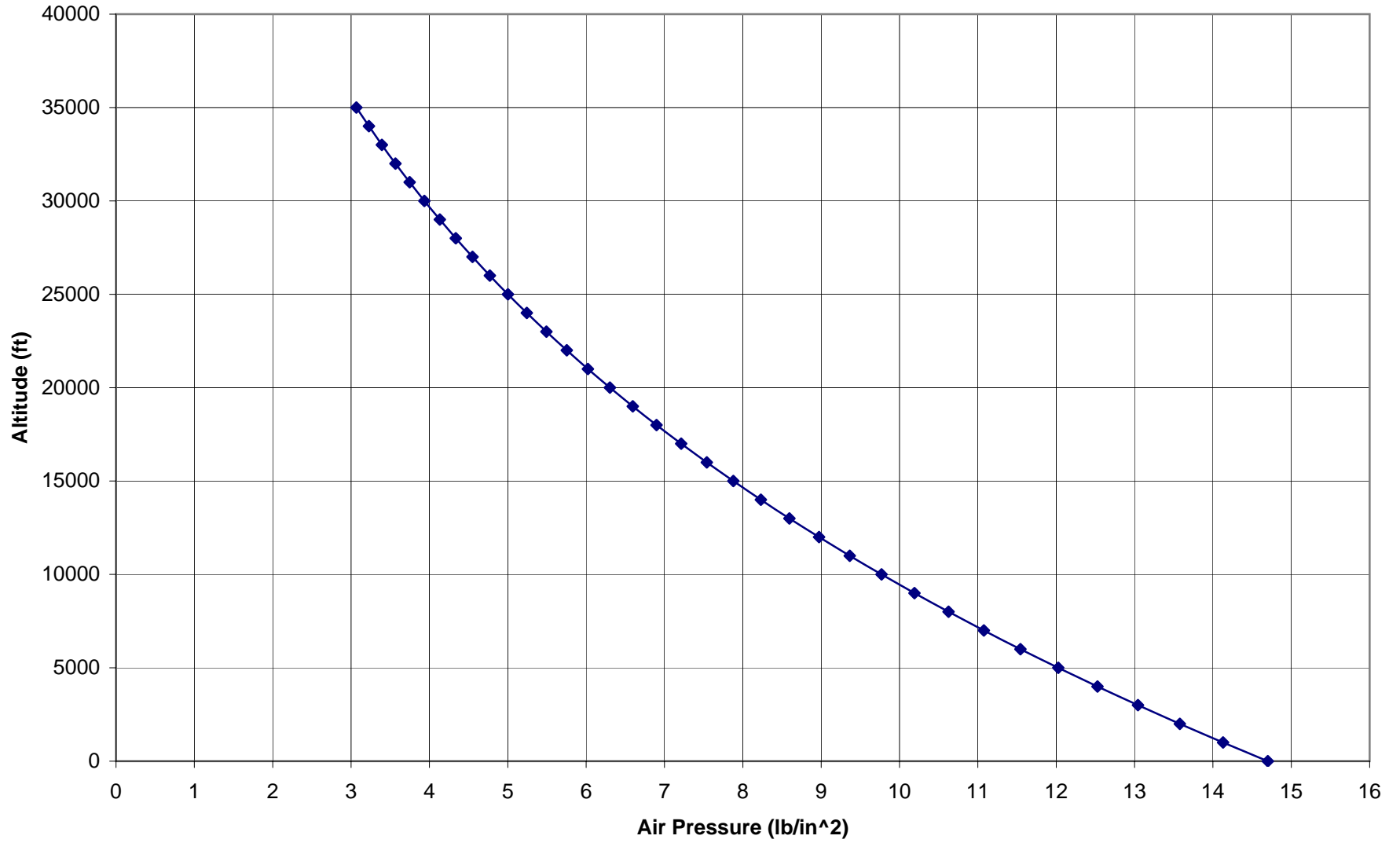
Air Pressure Activity – Air Pressure vs. Altitude Graph
